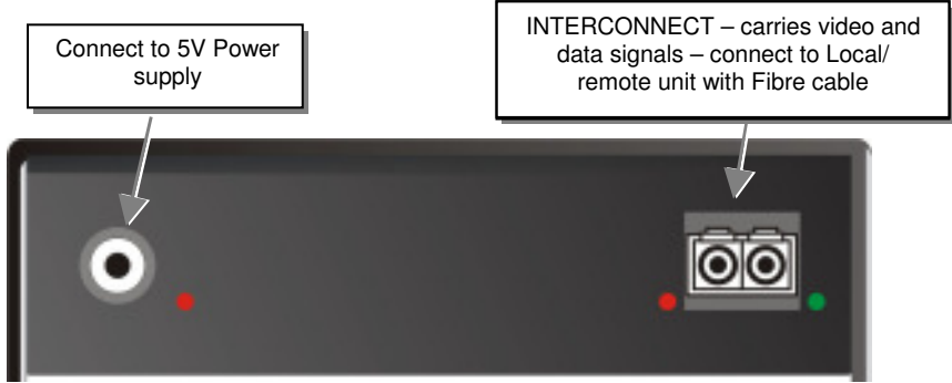
DVI-D KVM Extender KVM-Extender Type ACS1009A-xx Local/ Remote Unit
