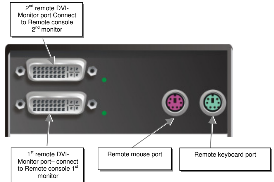
DVI-D KVM Extender KVM-Extender Type ACS2209A-xx Remote Unit
