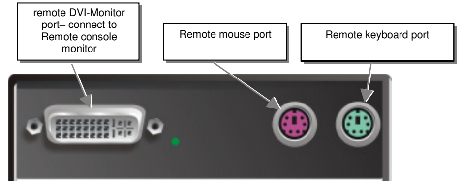
DVI-D KVM Extender KVM-Extender Type ACS1009A Remote Unit
