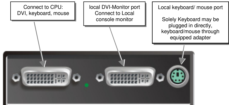
DVI-D KVM Extender KVM-Extender Type ACS1009A Local Unit
